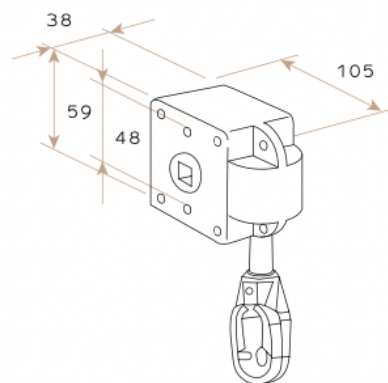
GEARBOX 7:1 (mm)
