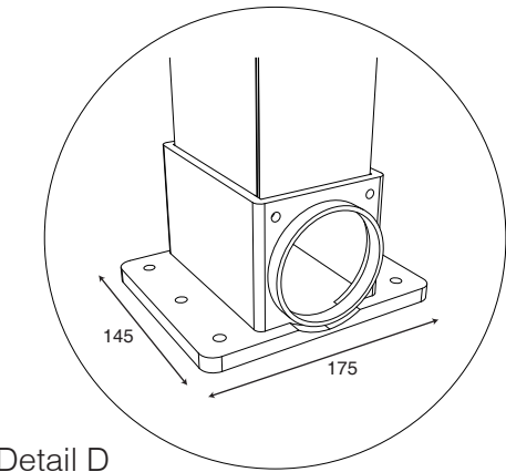
Detail D
